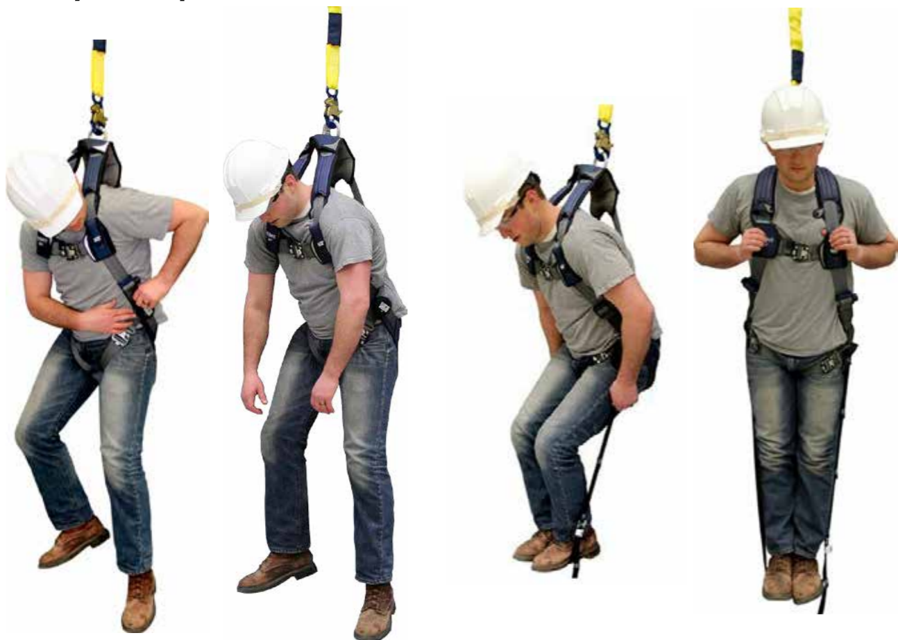
Step 1: Unzip packs to deploy Step 2: Pull out straps and hook Step 3: Put foot into web loop Step 4: Stand up relieve pressure
